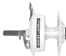
X-SD [S/C/B] THH50 L 70mm Left Drum Brake Hub S [Solid Axle 130mm] C [Solid Axle 100mm] B [Solid Axle 90mm]
